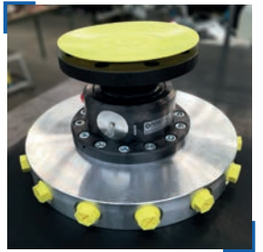
ROTARY UNION WITH 1 INLET AND 14 OUTLETS, AERONAUTICAL SECTOR
